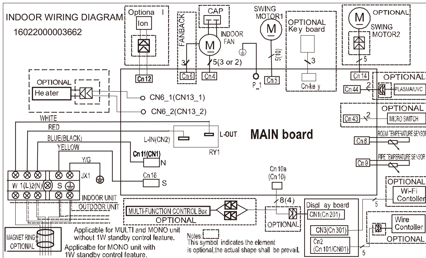
Indoor Unit IM2-XY 20M-70M / IL3-XY 20M-70M
