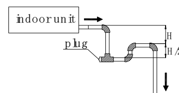
Figure 3-6.6: Drain piping water traps
