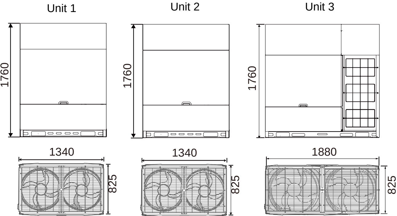
Figure 2-2.10: 74/76/78/80HP dimensions (unit: mm)
