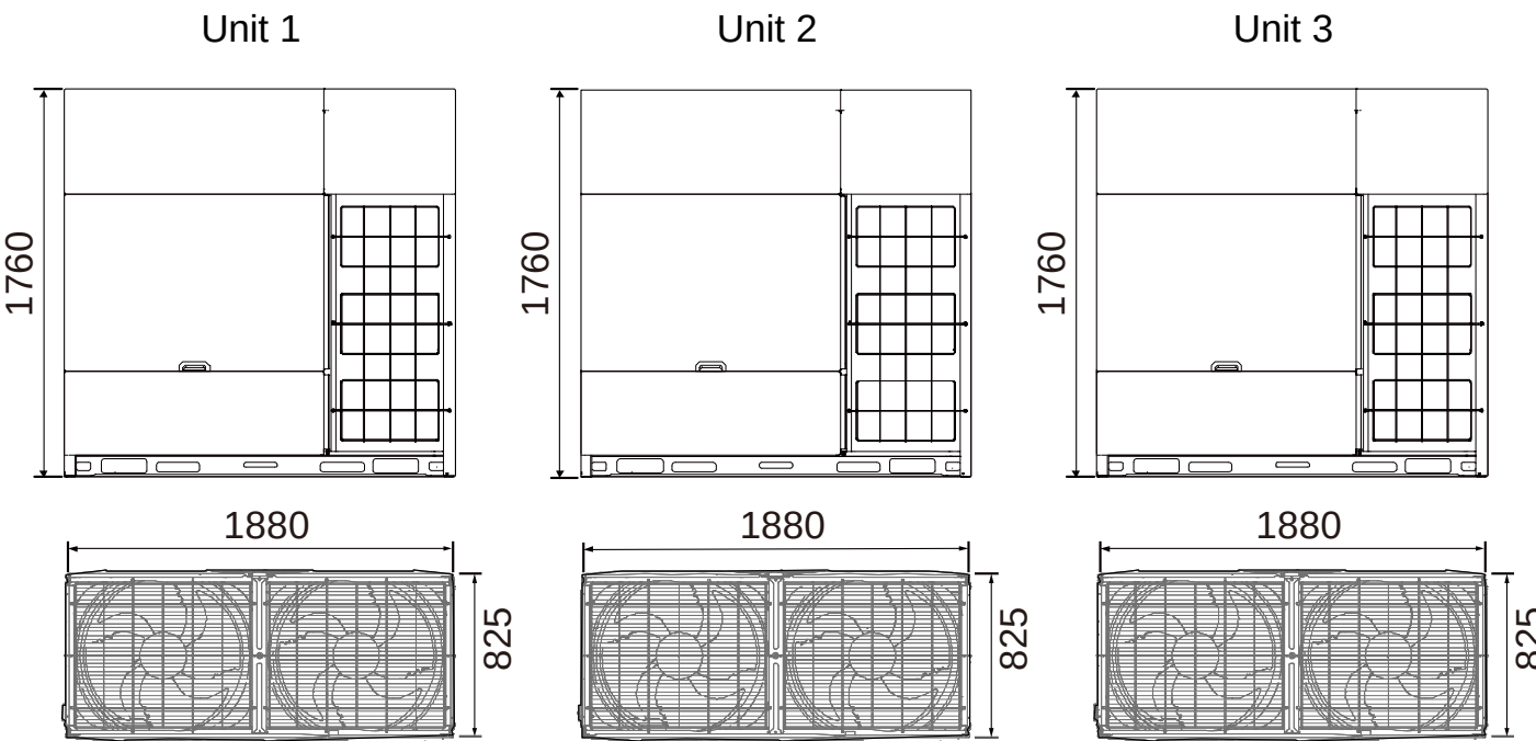
Figure 2-2.12: 90/92/94/96HP dimensions (unit: mm)
