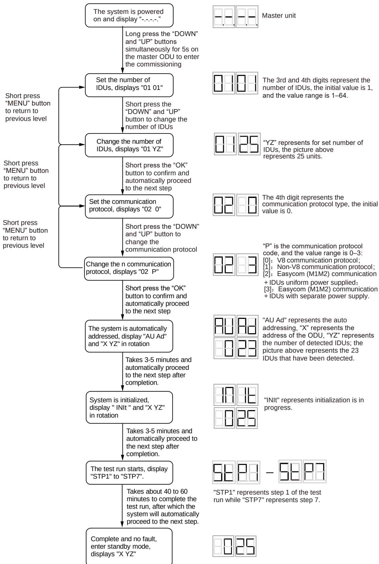
Figure 3-11.1: Commissioning Procedure
