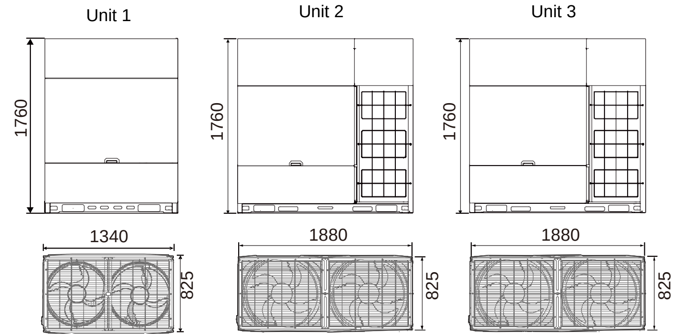
Figure 2-2.11: 82/84/86/88HP dimensions (unit: mm)
