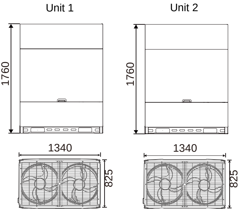
Figure 2-2.6: 42/44/46/48HP dimensions (unit: mm)
