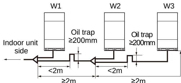
Figure 3-5.11: Oil trap between outdoor units
