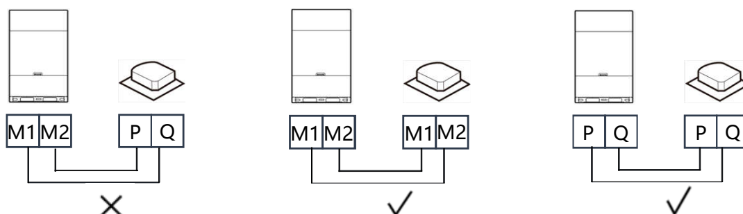
Figure 3-9.5: Communication wiring
