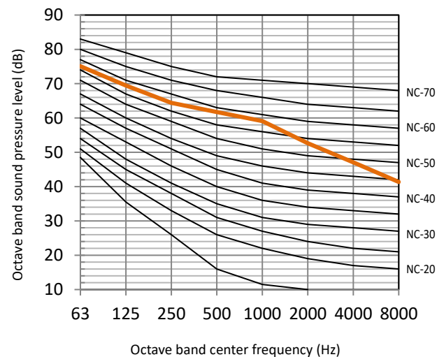
Figure 2-10.7: 18HP octave band level
