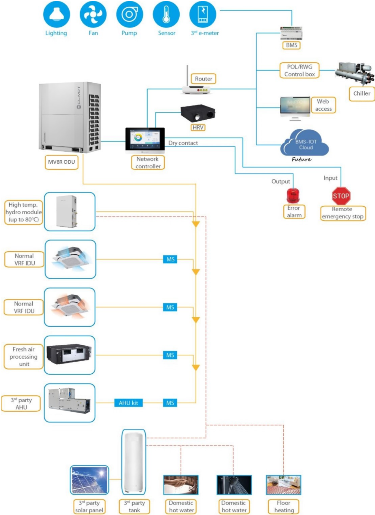
Figure 3.1: Hydraulic box connection method
