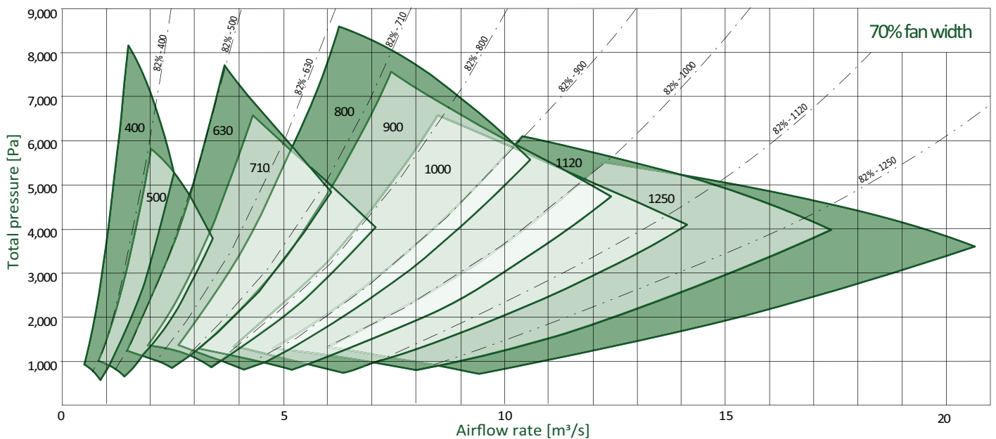
Performance curves
