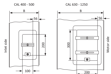
Dimensions of inspection hatches
