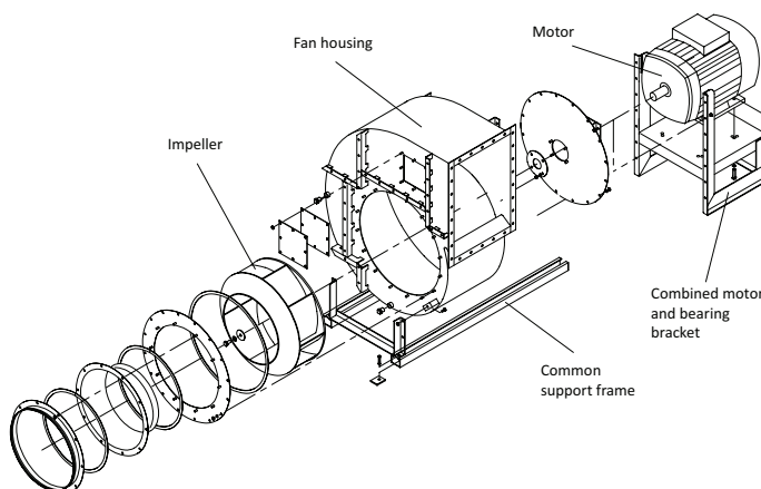
Exploded view of the CAL
