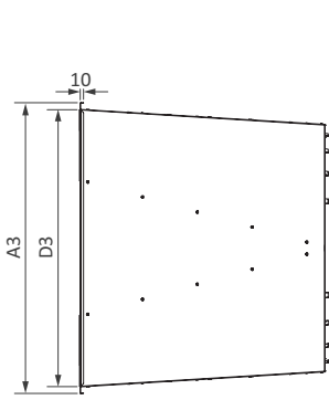
Round-to-square diffuser
