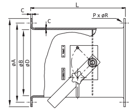
Damper type SBC
