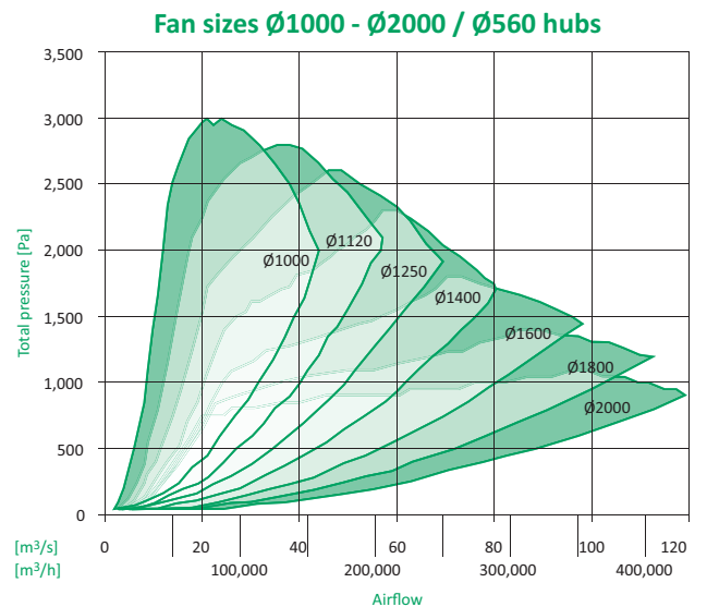
Specific performance curves for fans with frequency converters
