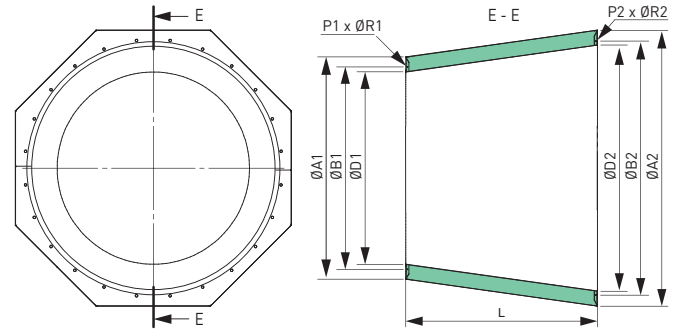
Type YAZ without core
