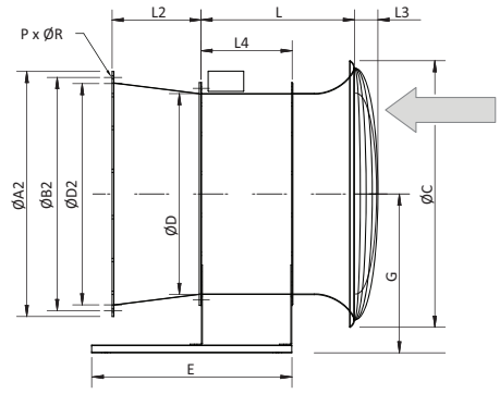
Support frame, inlet cone and round diffuser for AZN
