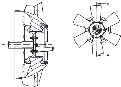
AZN 1000 impeller with Ø560 hub
