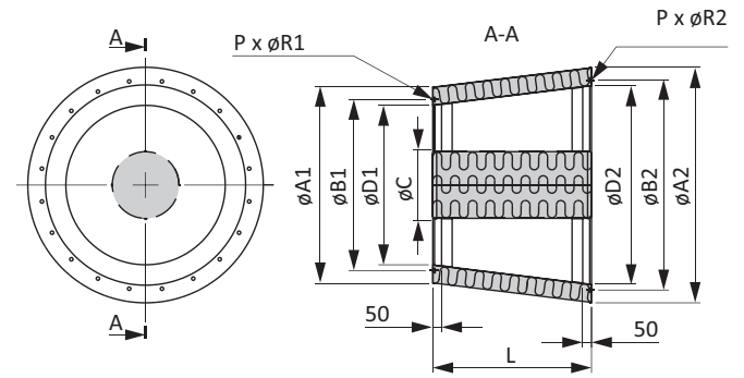
Type YAD with core
