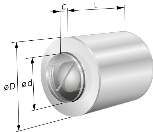
Figure 5. SORDO-P – Dimension print
