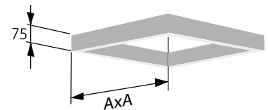
Figure 8. SAR K frame. When installing size 315-600 and 400-600 diffusers, position the ALS box so that its branch extends 20 mm below the ceiling surface.
