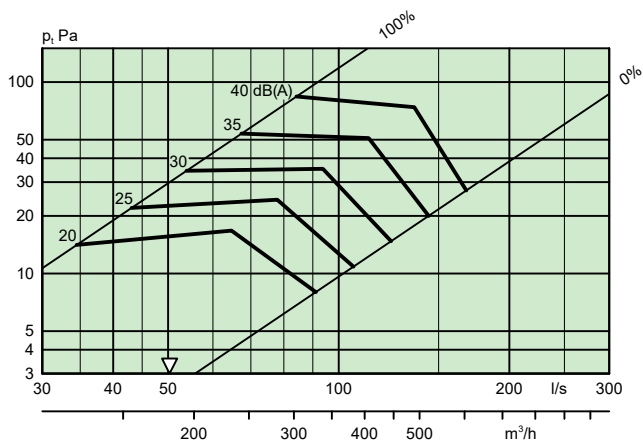
SWAN ACT 4-1158 + SWAN T 4-200
