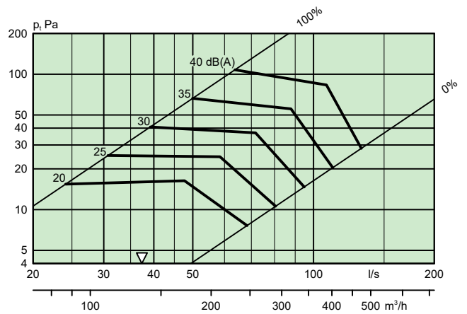
SWAN ACT 4-1158 + SWAN T 4-160
