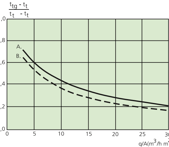
Diagram 3. Sizeless temperature difference in the floor zone at different airflows. A = \alpha_{kg} = 5 \text{ W}/(\text{m}^2 \cdot \text{K}) (thermal exchange constant due to convection on the floor surface). B = \alpha_{kg} = 3 \text{ W}/(\text{m}^2 \cdot \text{K})
