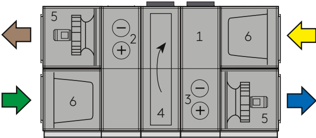
Principle for the air handling unit, complete with integrated reversible heat pump 1) Reversible heat pump section including compressor, 4-way valve, etc. 2) Exhaust air coil cooling/heating 3) Supply air coil cooling/heating 4) Rotary heat exchanger (Sorption rotor) 5) Fan 6) Air filter
