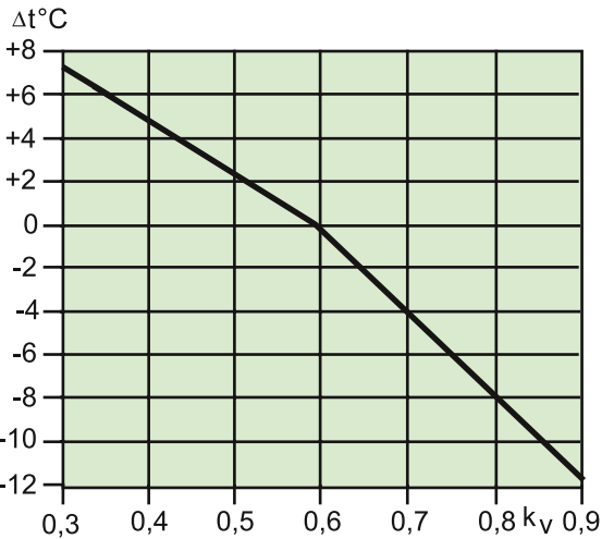
The relationship between the correction factor k_v and the temperature difference \Delta t °C (t supply air – t extract air ).
