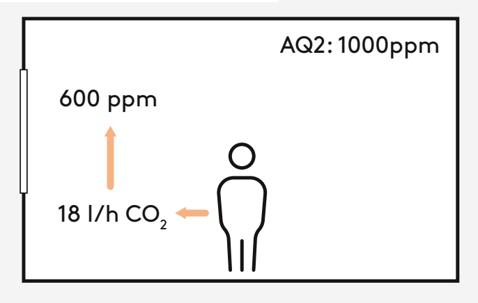
The requisite airflow for an office where sedentary work is performed and with air quality AQ2
