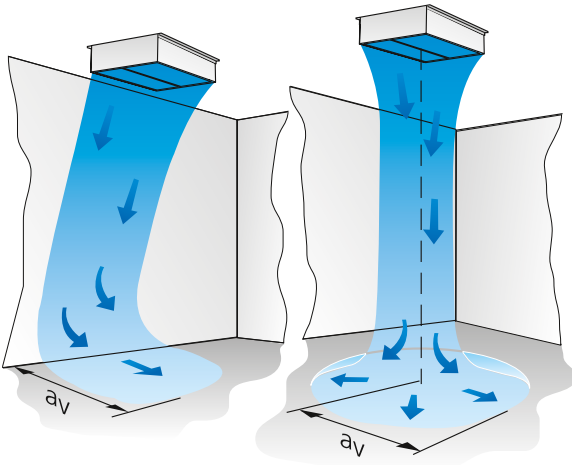
Ceiling mounted low velocity diffusers
