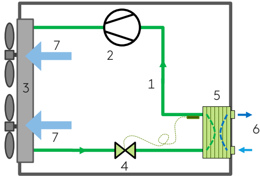
Principle for air-cooled water chiller 1) Refrigerant 2) Compressor 3) Condenser with fans 4) Expansion valve 5) Evaporator (heat exchanger) 6) Cooling agent (water) 7) Ambient air
