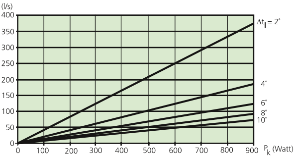
Max. airflow as a function of the cooling load.
