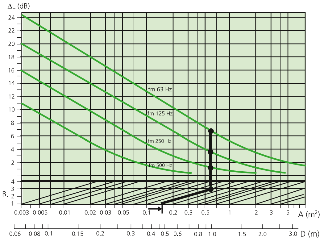
Sound attenuation \Delta L = Attenuation (dB) B = Placement of the duct opening (see illustration above to the right) A = Cross-sectional area of the duct with rectangular cross section (m²) D = Opening diameter for ducts with circular cross section (m)
