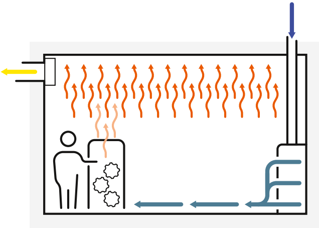
Displacement ventilation
