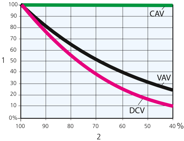
Relative energy use depending on type of system. 1. Relative energy use fan (%) 2. Relative airflow requirement (%) CAV = Constant Air Volume VAV = Variable Air Volume DCV = Demand Controlled Ventilation
