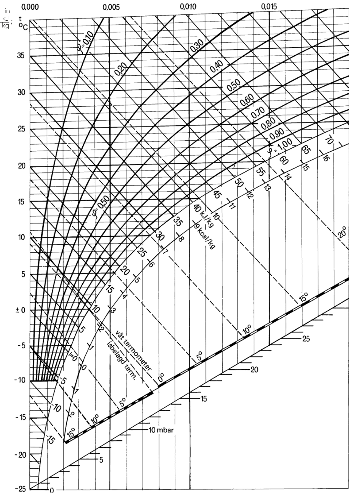
Mollier diagram for humid air -25 to +40 °C
