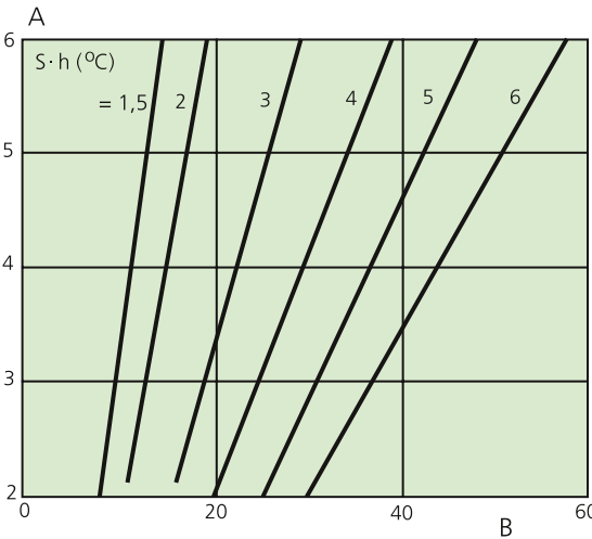
Diagram 1. The required ventilation flow as a function of the cooling capacity for different products of gradient and room height. A = Airflow (l/s,m 2 ) B = Cooling capacity (W/m 2 )
