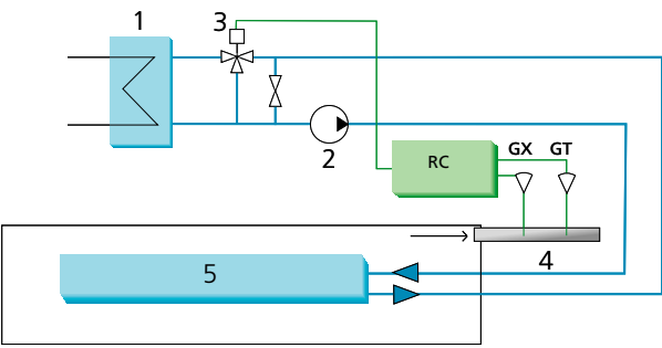
Condensation protection control via the shunt group. 1 = Evaporator/condenser 2 = Circulation pump 3 = Shunt 4 = Extract air duct 5 = Chilled beam RC = Regulator GX = Humidity sensor GT = Temperature sensor
