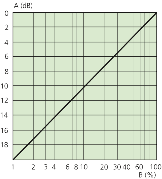
The relationship between the % branched air and attenuation A = Attenuation (dB) B = Air volume to room/terminal (%)
