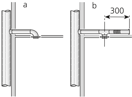
Counteracting crosstalk a) Low sound insulation b) High sound insulation. High attenuation can be obtained especially at duct lengths of 1-3 m.
