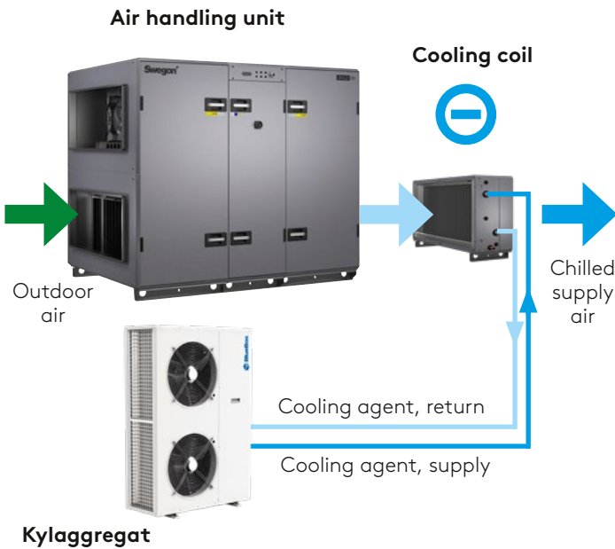
A typical application example within comfort ventilation is that the chiller supplies the air handling unit's cooling coil with chilled liquid.
