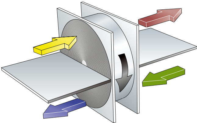
Rotary heat exchanger
