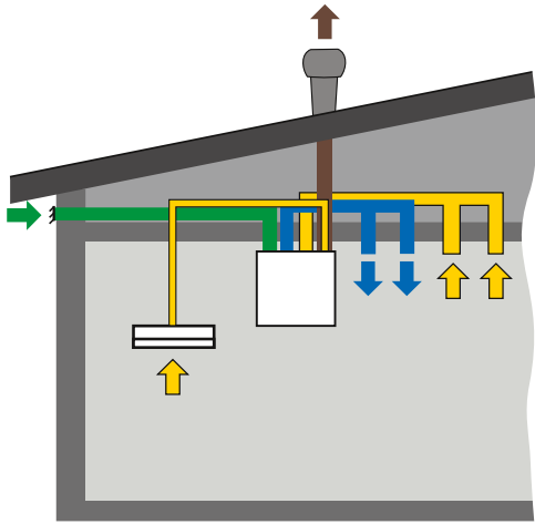
The solution with outside air via the facade, exhaust air to the exhaust hood, cooker hood attached to a ventilation unit.
