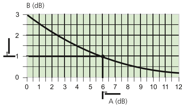
Logarithmic addition of two different levels A = Difference between levels to be added (dB) B = Increase to be added to the higher level (dB)
