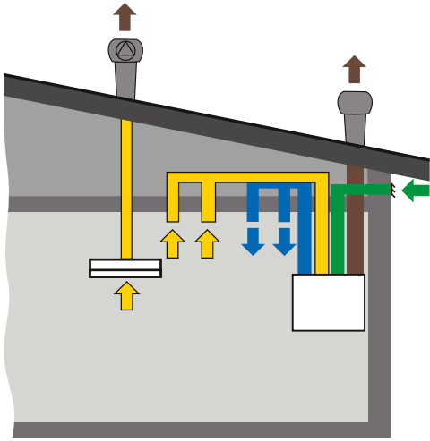
The solution with outside air via the facade, exhaust air to the exhaust hood, cooker hood attached to a roof fan (or fan of its own in the cooker hood).
