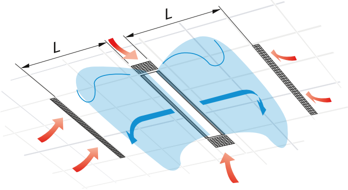
Recommended placement of circulation air openings in the suspended ceiling to the chilled beam
