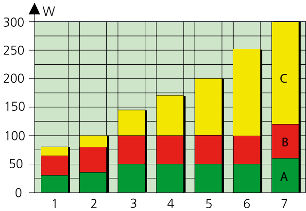
Heat emissions from the body during different types of work. A = Convection (green) B = Radiation (red) C = Evaporative emissions (yellow) 1 = Total rest 2 = Light office work 3 = Normal office work 4 = Computer work 5 = Light physical work 6 = Gentle walk 7 = Painting work
