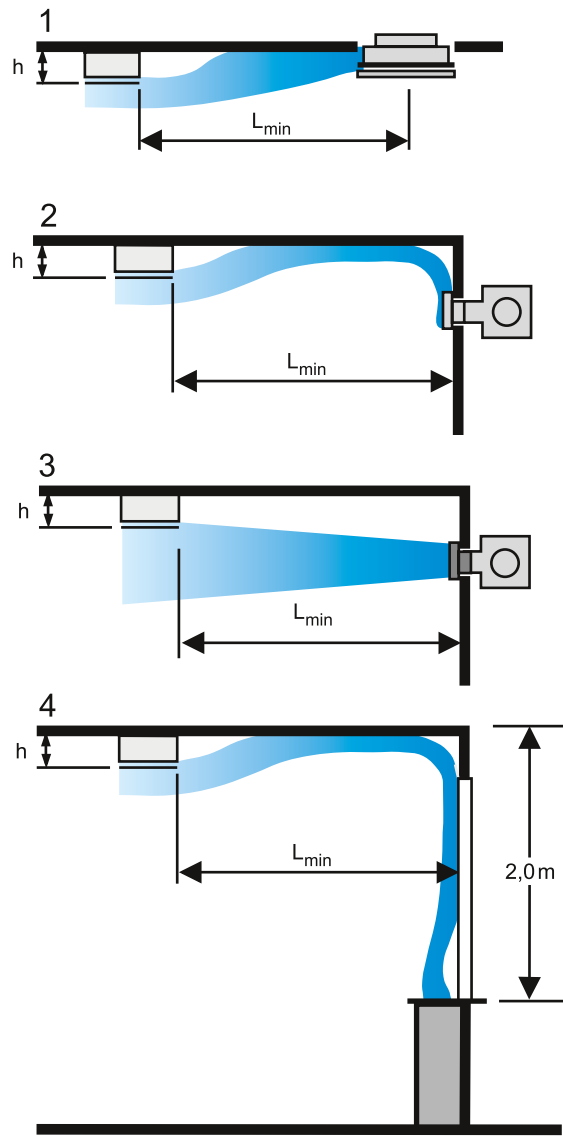
Different options for air supply with obstacles on the ceiling. 1 = Ceiling diffusers 2 = Rear edge diffusers 3 = Grilles in the wall 4 = Supply via window sill
