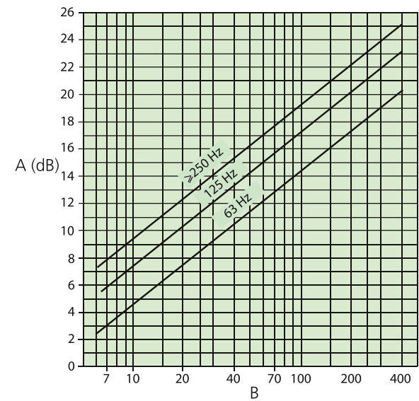
Attenuation in pressure and suction chambers internally lined with 100 mm thick mineral wool. (Note! The inlet and outlet must not be placed opposite to each other.) A = Attenuation (dB) B = Lined area divided by the outlet area.
