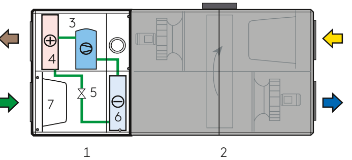
Principle for chillers with direct expansion docked to the air handling unit 1) Chiller 2) Air handling unit 3) Compressor 4) Condenser 5) Expansion valve 6) Evaporator 7) Air filter
