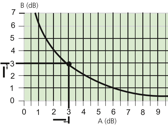
Logarithmic subtraction of two different levels A = Difference between total level and the level from sound source 1 (dB) B = Reduction to be subtracted from the total noise level (dB)
