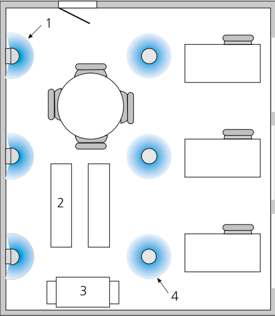
Diffuser placement in an open-plan office 1 = Concentration of supply air diffusers far from the workplace 2 = Book shelves 3 = Copying 4 = Alternative supply air diffuser in the form of “fake” pillars
