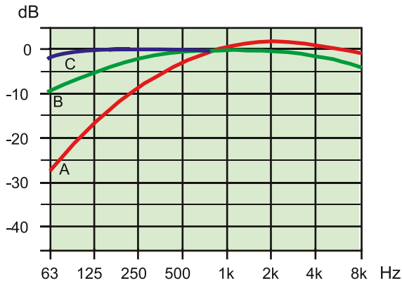
Attenuation for different weighting filters
