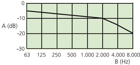
Octave band distribution of total sound power level in straight ducts A = Relative sound power level dB/octave (dB above 1 pW) B = Mean frequency octave band (Hz)
