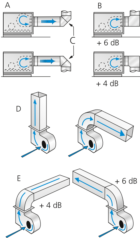
Examples of the right and wrong duct design after a fan A = Correct design B = Wrong design C = Elbow angled 45 degrees on the outside D = Correct design - duct elbow should be aligned with the fan's direction of rotation. E = Wrong design
