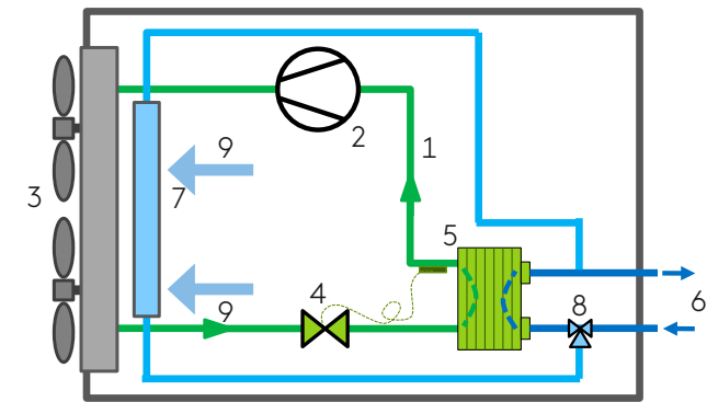
Principle for an air-cooled water chiller with free cooling 1) Refrigerant 2) Compressor 3) Condenser with fans 4) Expansion valve 5) Evaporator (heat exchanger) 6) Cooling agent (water) 7) Heat exchanger for cooling agent 8) Three-way valve for cooling agent return 9) Ambient air
