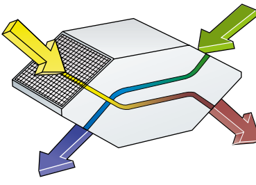
Counter-flow plate heat exchanger
