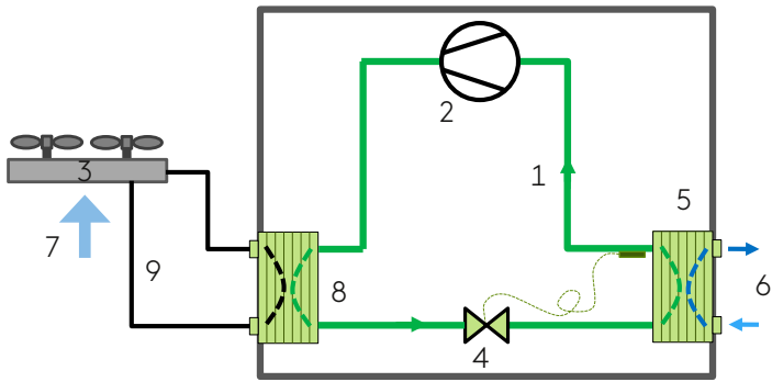
Principle for water-cooled water chiller 1) Refrigerant 2) Compressor 3) Outdoor dry coolers with fans 4) Expansion valve 5) Evaporator (heat exchanger) 6) Cooling agent (water) 7) Ambient air 8) Condenser/heat exchanger 9) Fluid circuit
