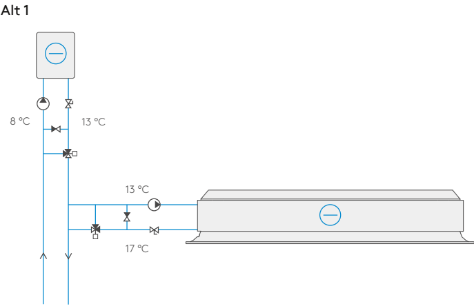
System principle with flows and temperatures.
