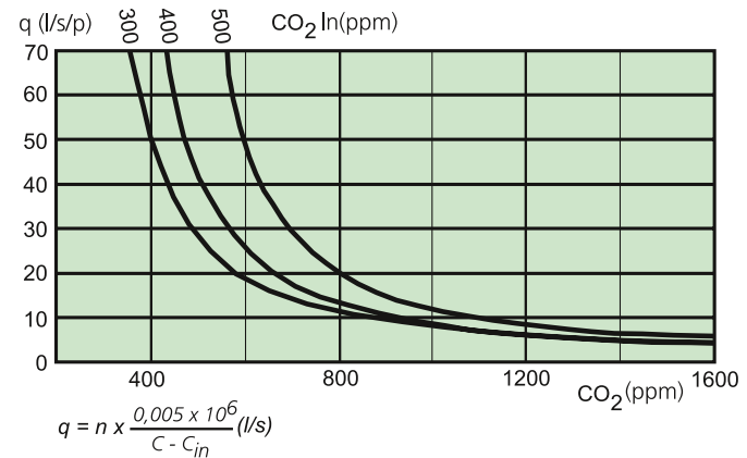
Max. airflow as a function of the air quality. (Seated persons, 70 kg)
