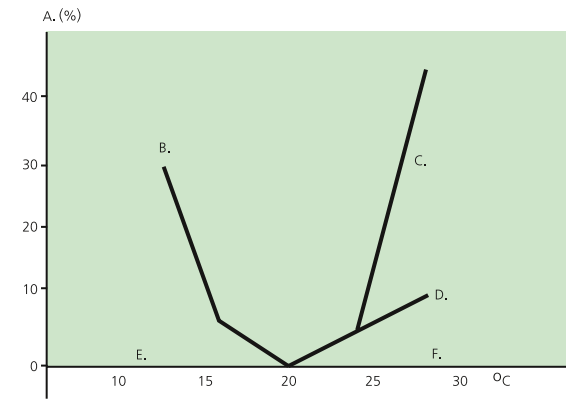
The accident rate for factory work changed with the indoor temperature (according to Wyon). A = Increase in the number of accidents in % B = Accidents C = Men D = Women E = Vigorous work (0.6 clo) F = Sedentary (1.0 clo)
