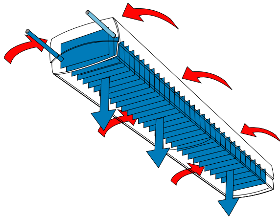
Principle of passive chilled beams
