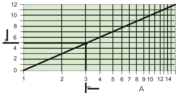
Logarithmic addition of several equal levels A = Number of sound sources B = Increase to be added to the level of the sound source, dB
