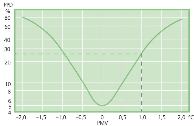
Expected percentage of dissatisfied (PPD = Predicted Percentage Dissatisfied) as a function of the thermal comfort experienced (PMV = Predicted Mean Vote). Example (dashed line): If the temperature is 1 degree warmer than the ideal temperature, 25% will be dissatisfied.
