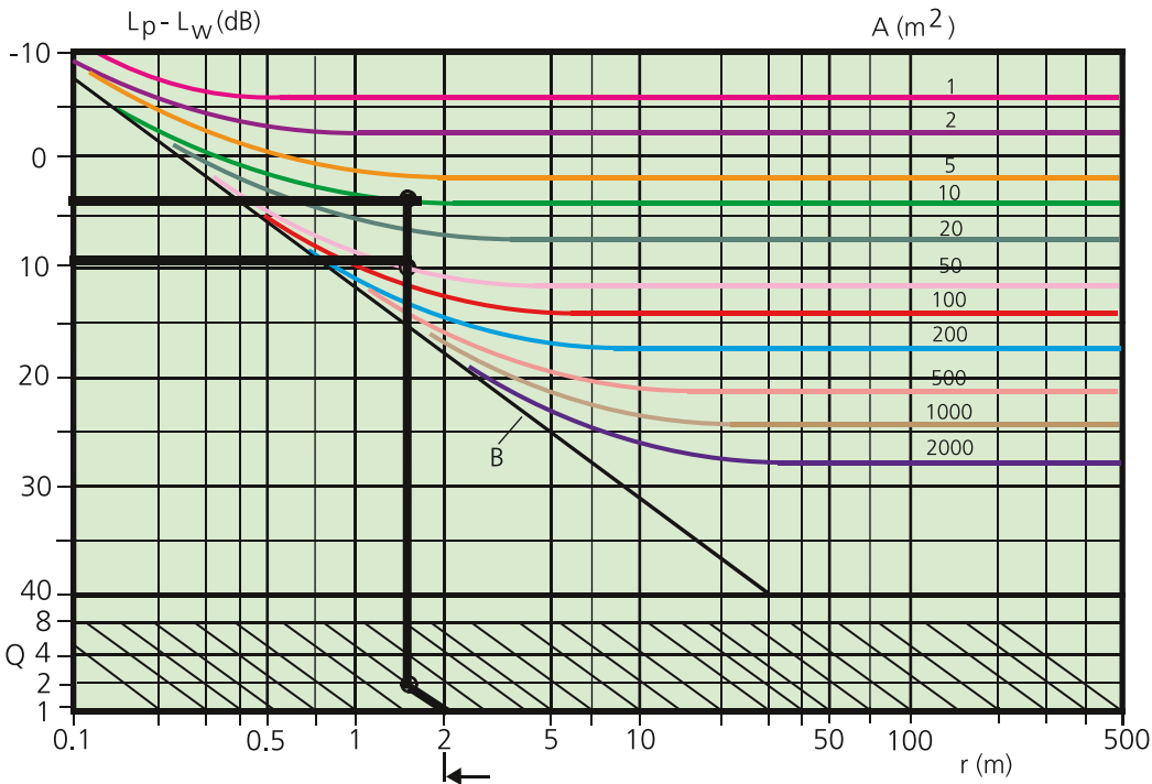
Difference between the sound power level and sound pressure level L p - L w = Difference between the sound power level and sound pressure level (dB). A = Equivalent sound absorption area (m 2 ) B = Free Field r = Distance from sound source (m)
