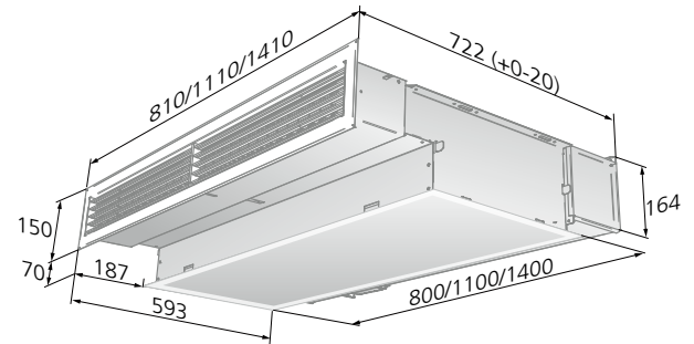
Figure 27. Dimensional drawing with grille
