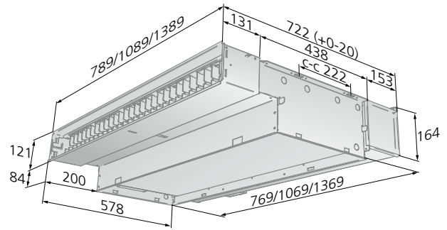
Figure 26. Dimensional drawing without grille
