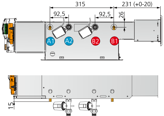
Figure 23. Dimensions water connection
