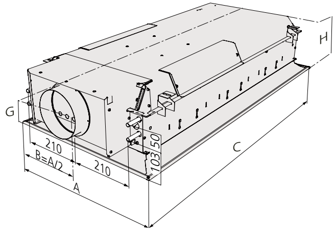
Figure 27. Dimensional drawing - short side connection (the length 1200 with air connection on side 1 is shown in the example).
