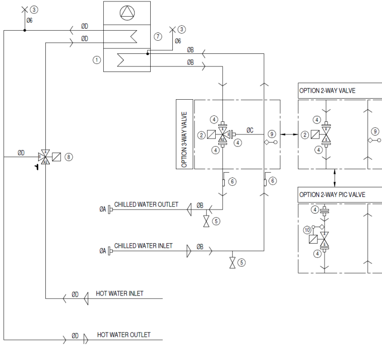
Single chilled water circuit
