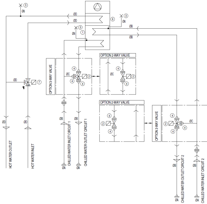
Single chilled water circuit
